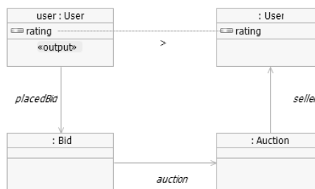
Figure 4. QQBE expression involving the comparator construct (“get users who used to bid for items sold by users with a lower rating”).
