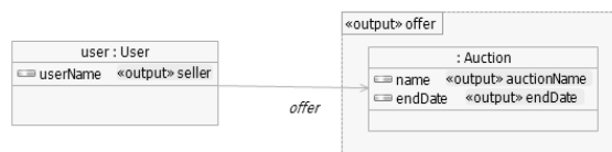
Figure 5. QQBE expression with a nested structure result (“get user names together with sets of names and end dates of their auctions”).
